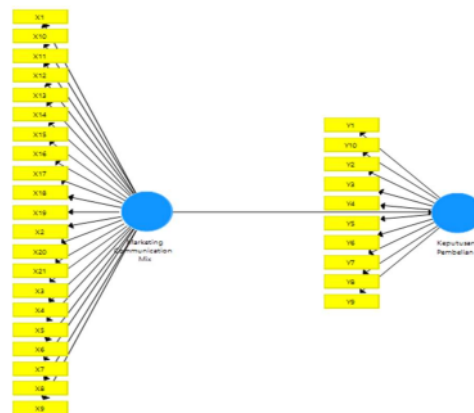
Fig.1. Measurement Model
